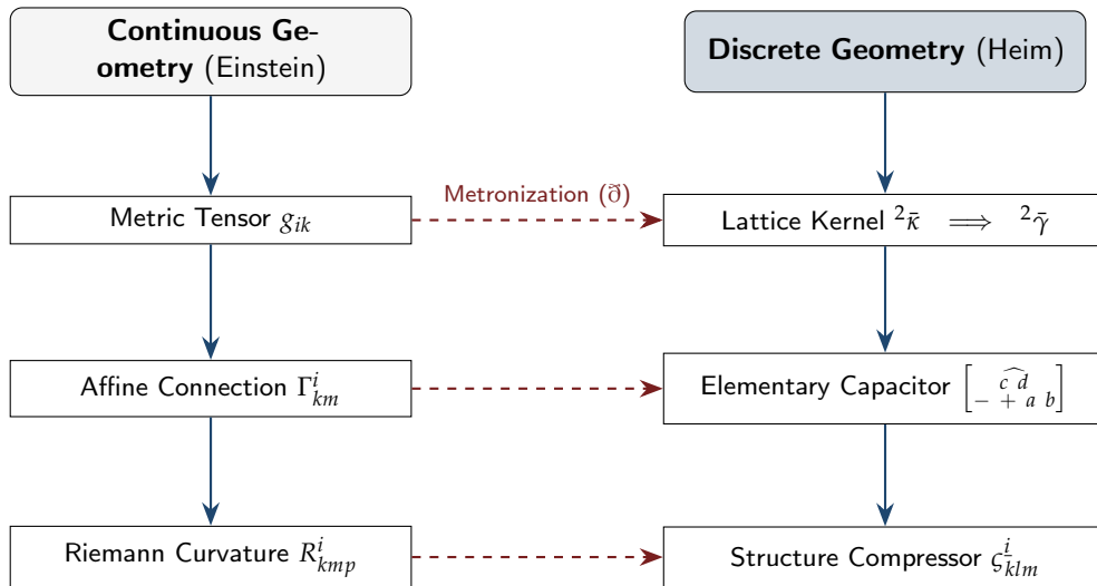
Figure 16: The translation of continuous General Relativity into Heim's discrete Metron Selector Theory.
