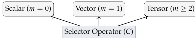
Figure 22: Hierarchical Structure of Selectors acting on Metron Functions.
