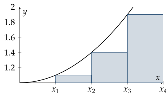
Figure 21: Discrete metronization of an integral area.
