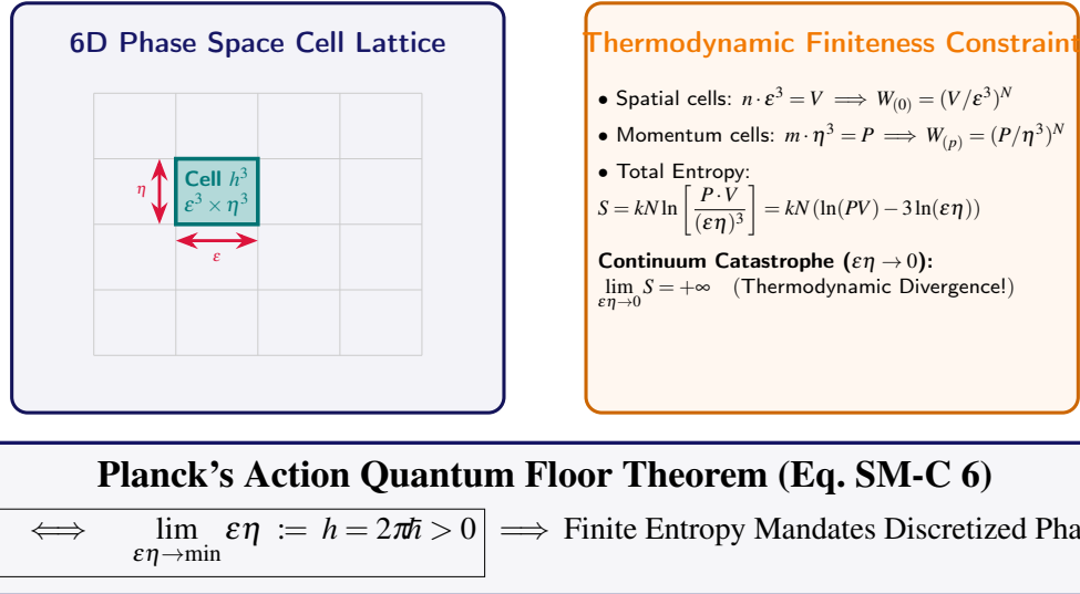
Figure 1.3. The Phase-Space Quantum Floor: Partitioning continuous phase space into elementary volume cells of action size \epsilon \eta \geq h to eliminate logarithmic entropy divergence.
