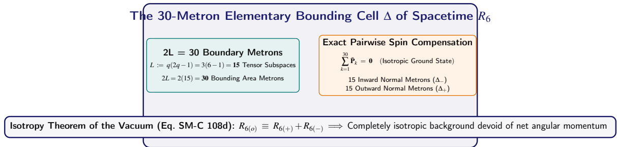
Figure 7.2. The 30-Metron Elementary Bounding Cell \Delta : Comprising 2L = 30 boundary metrons in pairwise spin balance to maintain vacuum isotropy.
