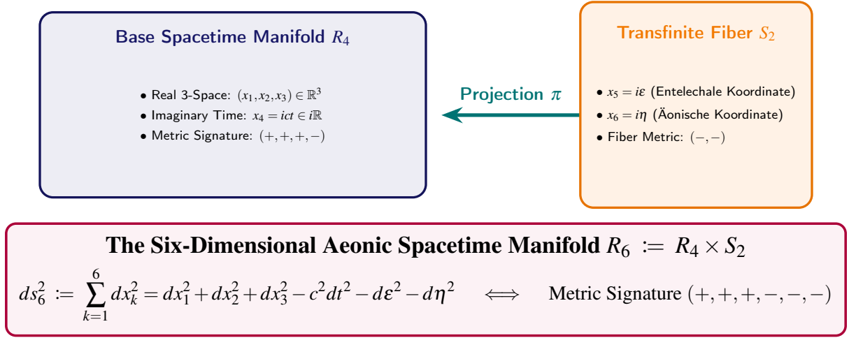
Figure 5.1. The Six-Dimensional Fiber Bundle Topology R_6 = R_4 \times S_2 : Base physical spacetime R_4 coupled to the 2D imaginary transfinite fiber S_2(i\varepsilon, i\eta) .
