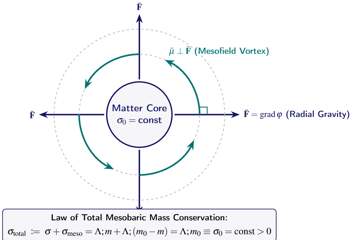
Figure 2.5. The Geometric Orthogonality of the Mesofield: Radial gravitational gradient field \bar{F} coupled to orthogonal rotational mesofield vortices \bar{\mu} .
