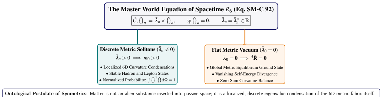
Figure 5.6. The Master World Equation: Mapping discrete metric curvature eigenstates \bar{\lambda}_n to stable elementary particles.
