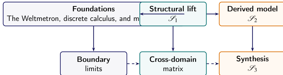
Figure 6.8. Deductive progression of Chapter VI.
