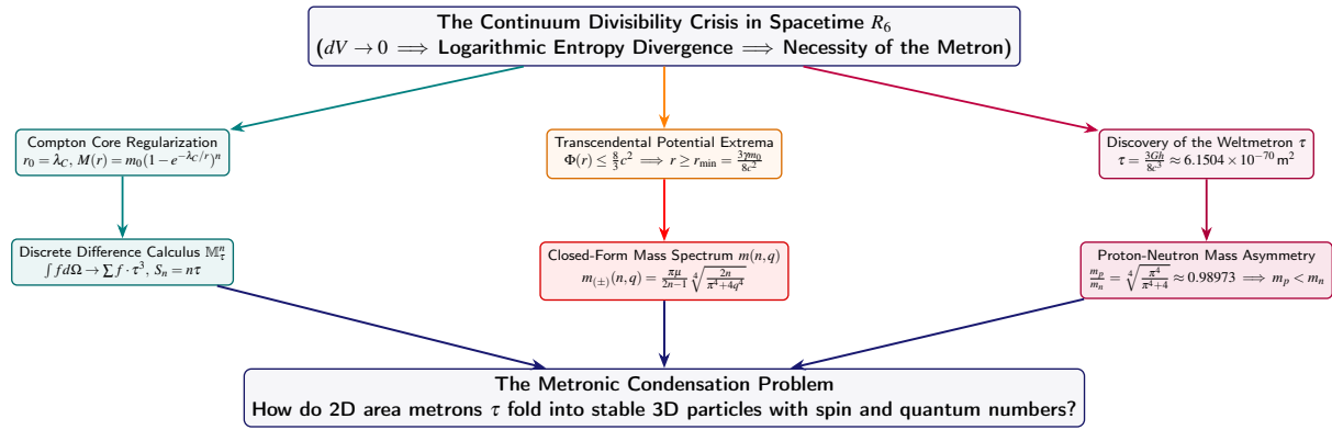
Figure 6.7. The Conceptual Deduction Tree of Chapter VI: From the continuum divisibility crisis to the Weltmetron \tau and the discrete elementary particle mass formula.
