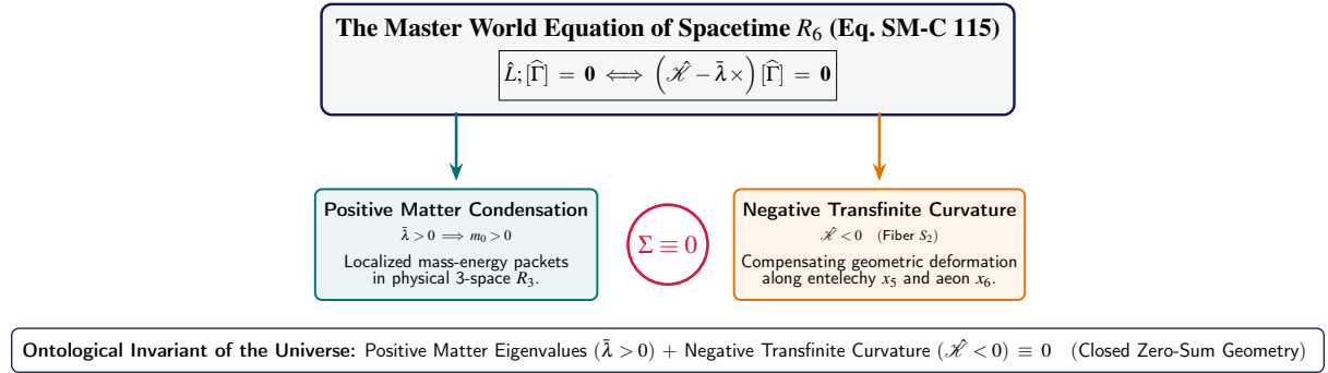
Figure 7.5. The Master World Selector Null-Hamiltonian: Proving that every positive matter condensation in R_3 is balanced by negative transfinite curvature in (x_5, x_6) .
