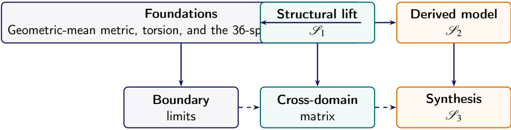
Figure 4.9. Deductive progression of Chapter IV.
