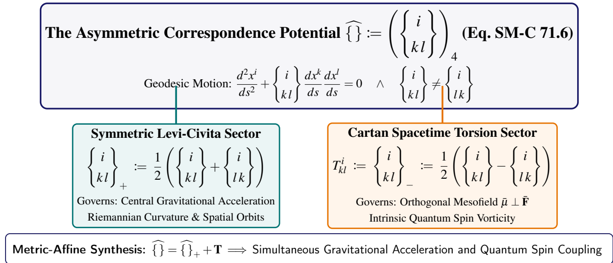
Figure 4.2. The Decomposition of the Asymmetric Correspondence Potential: Splitting into the symmetric Riemannian Levi-Civita connection \widehat{\{\}}_+ and the Cartan spacetime torsion tensor \mathbf{T} .
