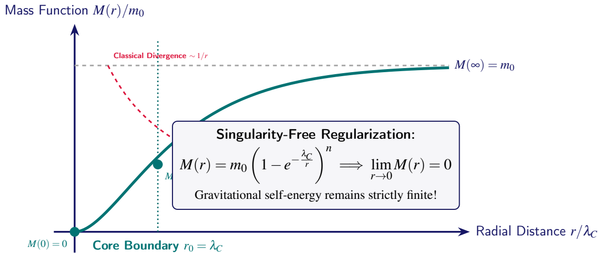
Figure 6.1. The Regularized Radial Mass Profile M(r) : Eliminating point-mass singularities via the Compton standing-wave core r_0 = \lambda_C .
