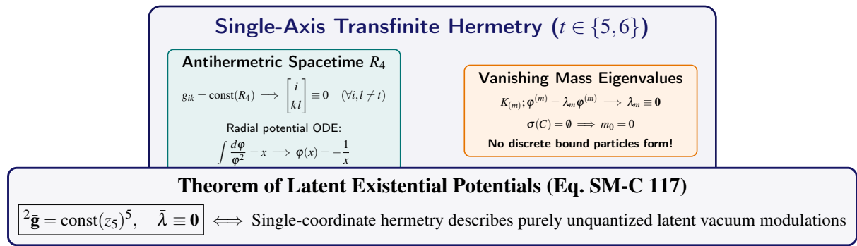
Figure 8.1. The Latent Potential Mechanism: Single-coordinate transfinite hermetry generates vanishing mass eigenvalues ( \lambda_m \equiv 0 ), acting as a continuous background potential.
