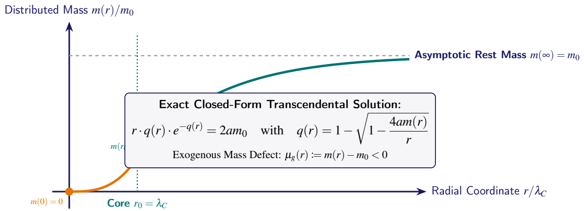
Figure 2.2. The Non-Linear Binet Mass Distribution Curve: Smooth transition from the cubic endogenous core ( r \leq r_0 ) to the asymptotic rest mass m_0 .
