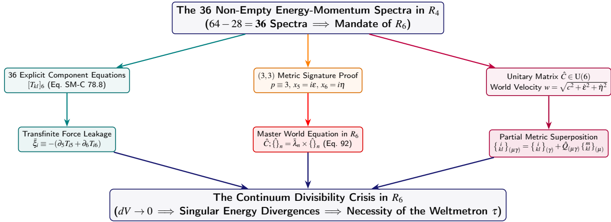
Figure 5.8. The Conceptual Deduction Tree of Chapter V: From the 36-component determination system to the 6D Master World Equation and the necessity of the Weltmetron.
