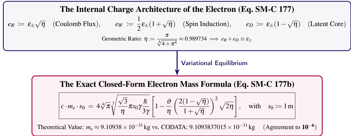
Figure 10.5. The Exact Electron Structure: Internal charge triad ( e_R, e_W, e_D ) and the parameter-free electron mass equation m_e .
