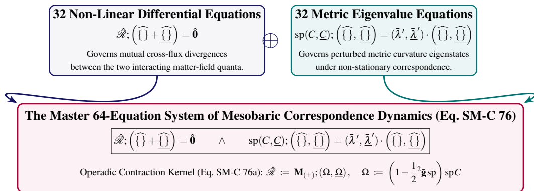
Figure 4.4. The Master 64-Equation Architecture of Mesobaric Correspondence Dynamics: Synthesizing 32 non-linear differential equations and 32 metric eigenvalue equations.
