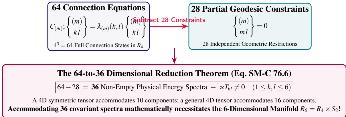
Figure 4.7. The 64-to-36 Dimensional Reduction: 28 partial geodesic constraints reduce the 64 connection equations to 36 physical energy spectra, mandating six-dimensional spacetime R_6 .
