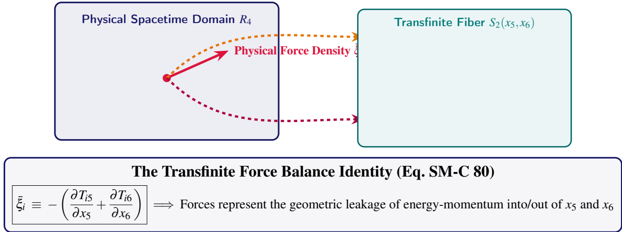
Figure 5.2. The Geometric Origin of Physical Force Fields: Observable 4D force densities \bar{\xi}_i as transfinite divergences along the entelechial and aeonic coordinates.
