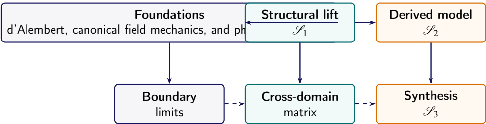
Figure 1.9. Deductive progression of Chapter I.
