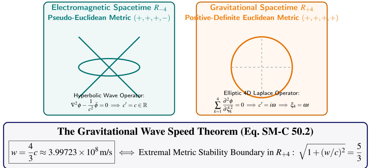
Figure 2.4. The Dual Spacetime Wave Metrics: Hyperbolic wave propagation in Minkowski spacetime R_{-4} versus elliptic Laplace propagation in Euclidean spacetime R_{+4} .
