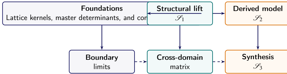
Figure 9.7. Deductive progression of Chapter IX.
