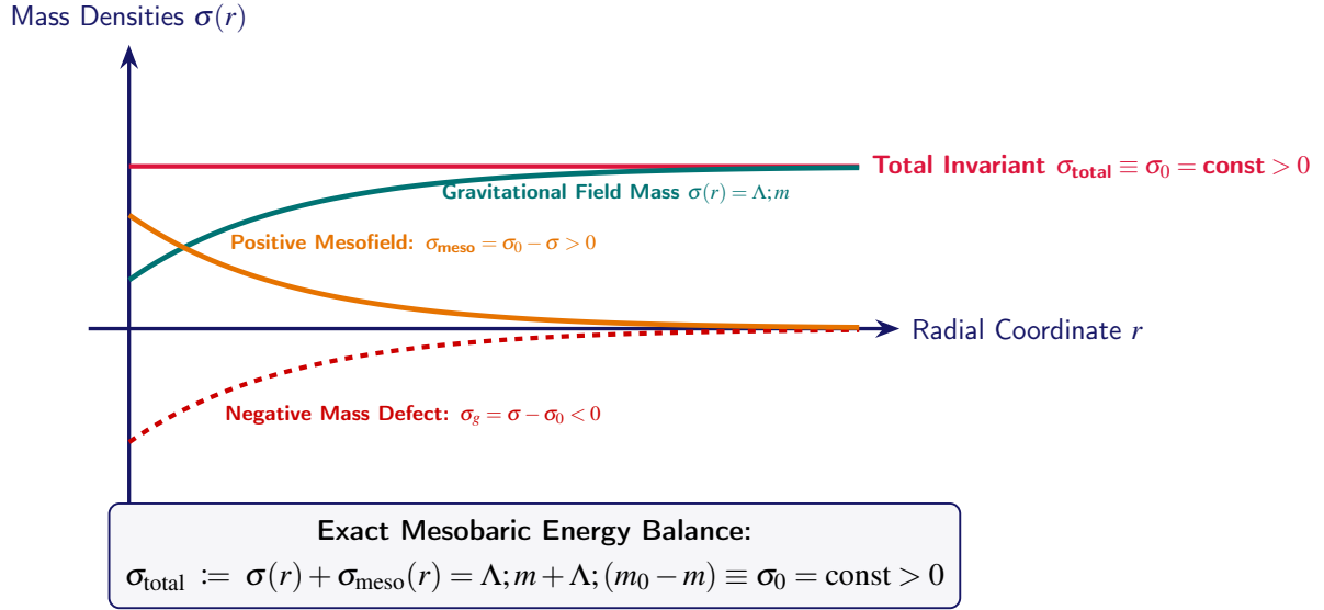
Figure 2.3. The Mesobaric Mass Compensation Mechanism: The positive-definite Mesofield \sigma_{\text{meso}} > 0 cancels the negative gravitational mass defect \sigma_g < 0 .
