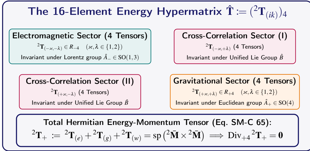
Figure 3.4. The 16-Element Block Architecture of the Energy Hypermatrix \hat{\mathbf{T}} : Decomposing into 4 Electromagnetic, 4 Gravitational, and 8 Cross-Correlation Tensors.
