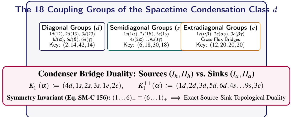
Figure 9.4. The 18 Coupling Groups of Type d Condensations: Categorized into Diagonal ( d ), Semidiagonal ( s ), and Extradiagonal ( e ) Groups with Exact Source-Sink Bridge Duality.
