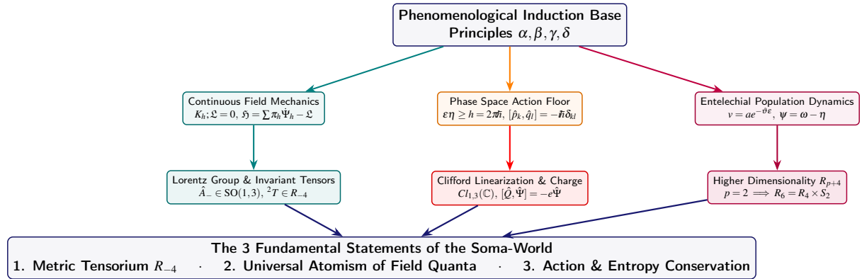
Figure 1.8. The Conceptual Deduction Tree of Chapter I: From the phenomenological induction axioms to the three fundamental statements of the Soma-World.
