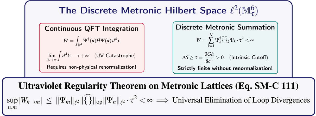
Figure 7.3. Ultraviolet Regularity on the Discrete Metronic Hilbert Space: Bounded cell area \tau > 0 replaces divergent continuous loop integrals with finite lattice sums.
