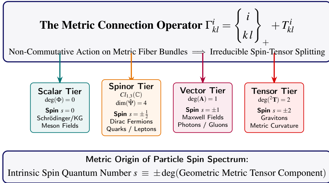
Figure 4.5. The Geometric Derivation of Particle Spin Spectra: Intrinsic spin s \in \{0, \pm \frac{1}{2}, \pm 1, \pm 2\} as an exact reflection of the tensor rank of metric connection components.
