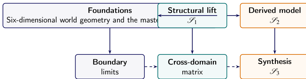
Figure 5.9. Deductive progression of Chapter V.
