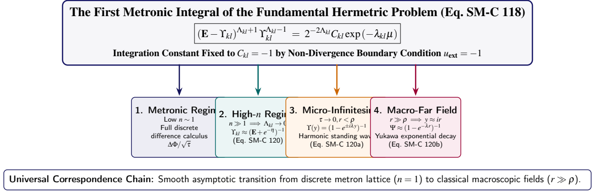
Figure 8.2. The Four Validity Regimes of the First Metronic Integral: Spanning the discrete metronic core ( n = 1 ) to classical Yukawa-like far fields.
