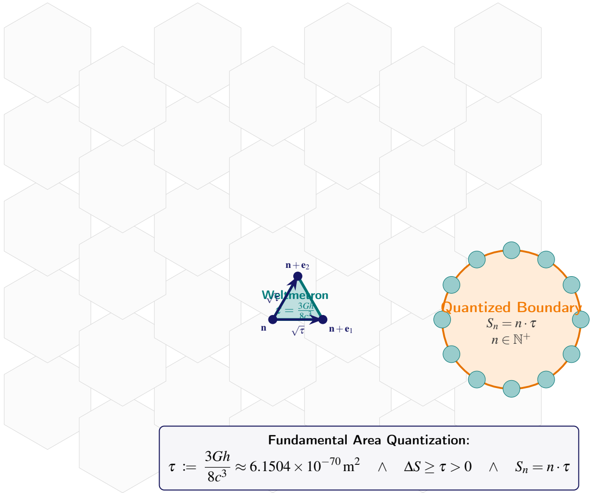
Figure 6.3. The Discrete Metronic Lattice Grid \mathbb{M}_{\tau}^n : Spacetime structured as a cellular network of indivisible two-dimensional area elements \tau = \frac{3Gh}{8c^3} .
