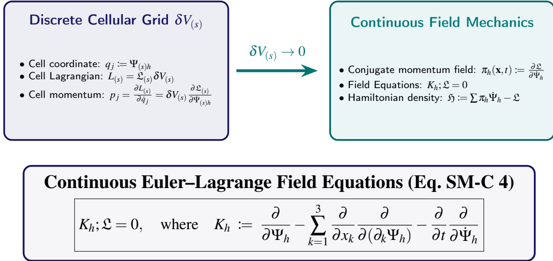
Figure 1.2. The Continuum Transition in Canonical Field Mechanics: Discretized cell volume \delta V_{(s)} converging to continuous Euler–Lagrange field densities.
