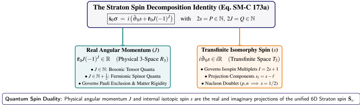
Figure 10.3. The Geometric Splitting of the Straton Spin: Real spatial angular momentum J in R_3 versus transfinite isomorphy spin s in T_3 .
