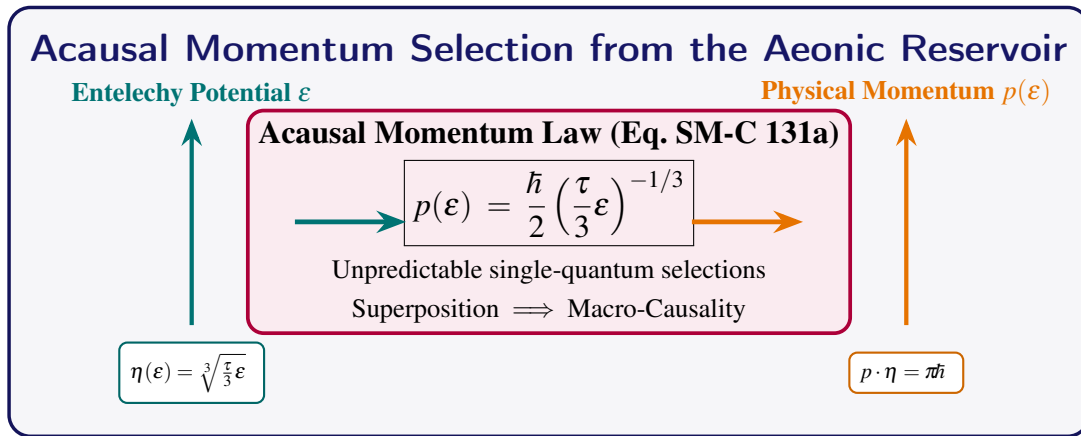
Figure 8.5. Acausal Momentum Actualization: Individual quantum selections from the aeonic reservoir of future potentials obey p(\varepsilon) = \frac{\hbar}{2}(\frac{\tau}{3}\varepsilon)^{-1/3} .
