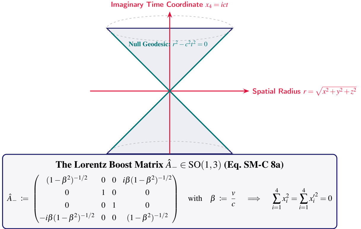
Figure 1.4. The Invariant Lightcone in Pseudo-Euclidean Spacetime R_{-4} : Spherical wave front invariance enforcing unitary Lorentz rotations \hat{A}_- \in SO(1,3) .
