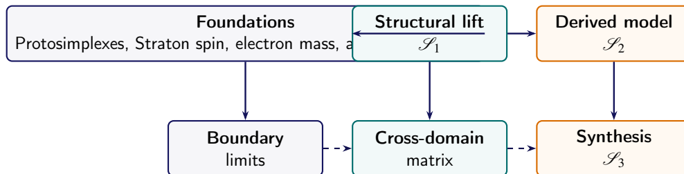
Figure 10.7. Deductive progression of Chapter X.
