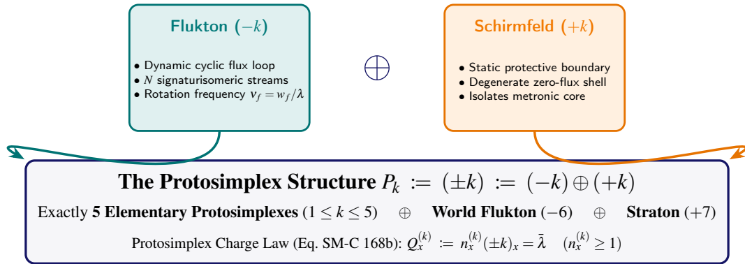
Figure 10.1. The Structural Synthesis of a Protosimplex: Coupling a dynamic cyclic Flukton ( -k ) with a static boundary Schirmfeld ( +k ).
