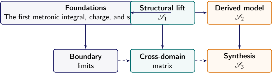
Figure 8.9. Deductive progression of Chapter VIII.
