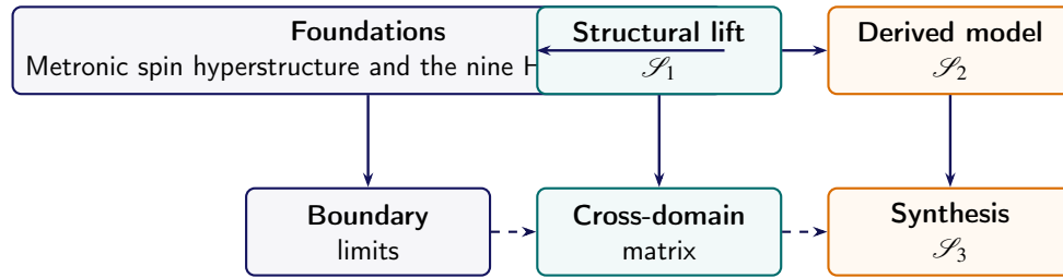
Figure 7.8. Deductive progression of Chapter VII.
