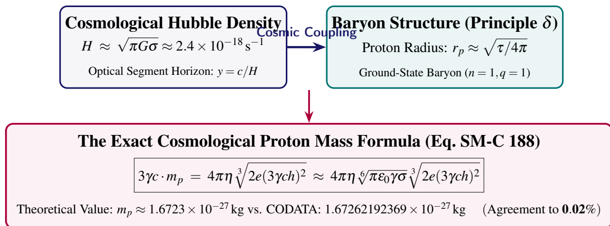
Figure 11.2. The Cosmological Proton Mass Coupling: Deducing the proton rest mass m_p directly from the Hubble expansion parameter H and universal constants.
