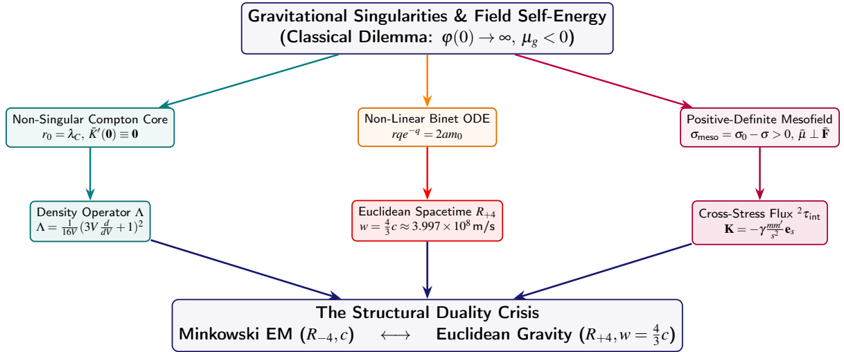
Figure 2.7. The Conceptual Deduction Tree of Chapter II: Resolving point singularities and mass defects, culminating in the structural duality crisis between R_{-4} and R_{+4} .
