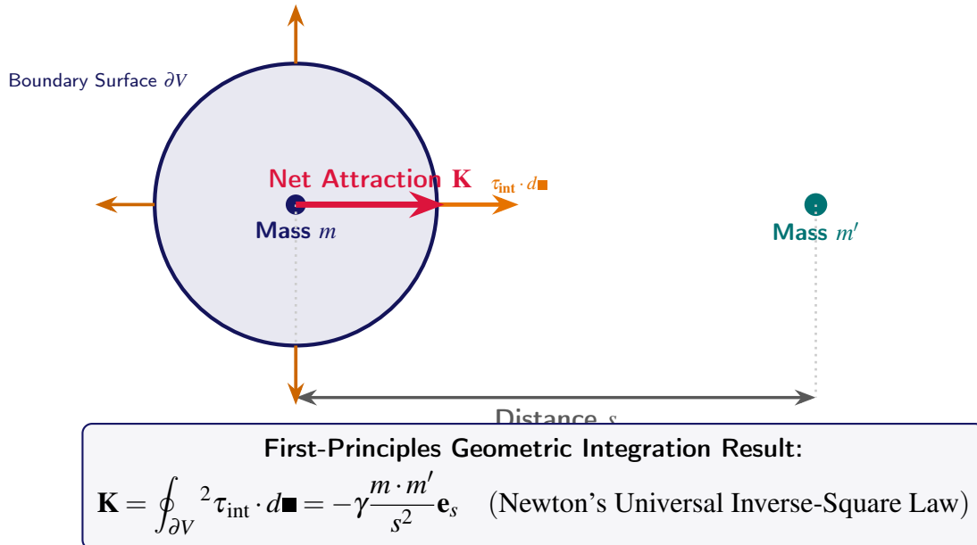
Figure 2.6. The Geometric Origin of Newton's Gravitational Law: Surface integration of the non-linear interaction cross-stress tensor {}^2\tau_{\text{int}} over the boundary \partial V .
