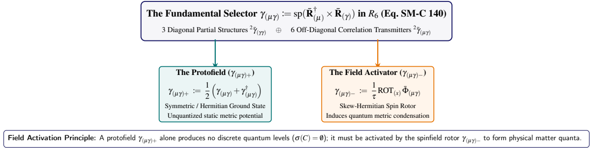
Figure 9.1. The Structural Splitting of the Fundamental Selector \hat{\gamma} : Decomposing into the symmetric static Protofield \gamma_{(\mu\gamma)+} and the anti-Hermitian Spinfeld Activator \gamma_{(\mu\gamma)-} .
