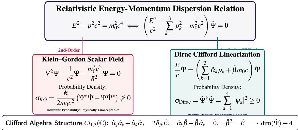
Figure 1.5. The Necessity of Clifford Linearization: Resolving Klein–Gordon negative probability densities via the 4-component Dirac spinor module Cl_{1,3}(\mathbb{C}) .
