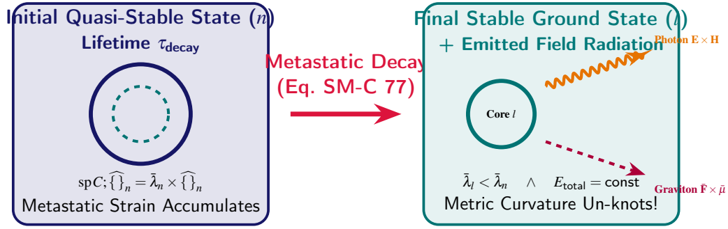
Figure 4.6. The Physics of Mesobaric Metastatics: Spontaneous particle decay and transmutation modeled as a topological un-knotting of the non-linear metric connection.
