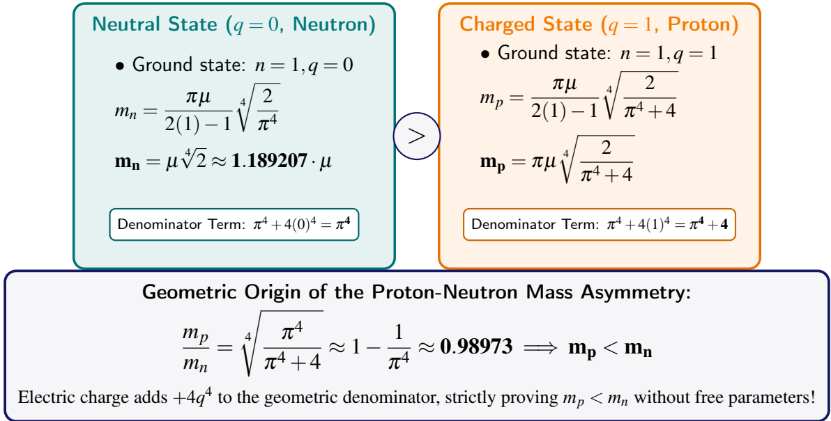
Figure 6.6. The Geometric Resolution of the Proton-Neutron Mass Asymmetry: Electrostatic charge q = 1 expands the metronic denominator, forcing m_p < m_n .
