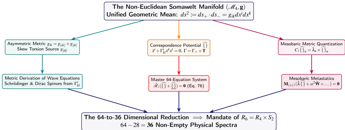
Figure 4.8. The Conceptual Deduction Tree of Chapter IV: Synthesizing non-Euclidean metrics, connection potentials, wave mechanics, metastatics, and the 6D spacetime mandate.
