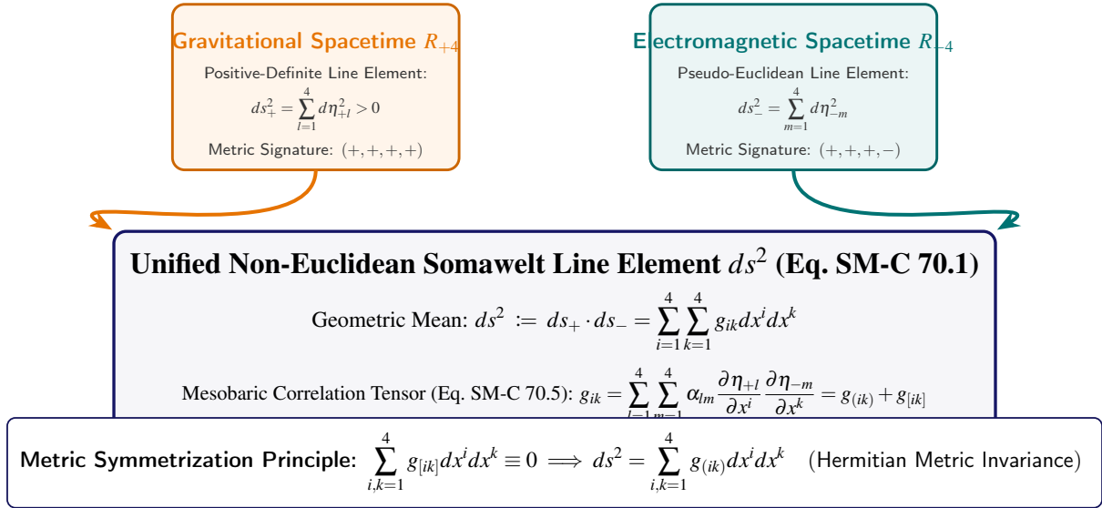
Figure 4.1. Construction of the Unified Non-Euclidean Somawelt Metric: Synthesizing the Euclidean gravitational interval ds_+ and Minkowski interval ds_- via the geometric mean ds^2 = ds_+ ds_- .
