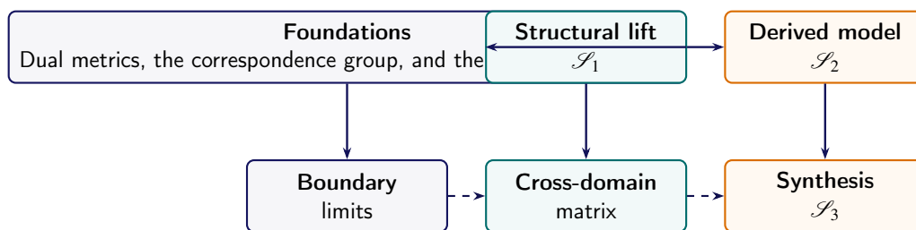
Figure 3.8. Deductive progression of Chapter III.
