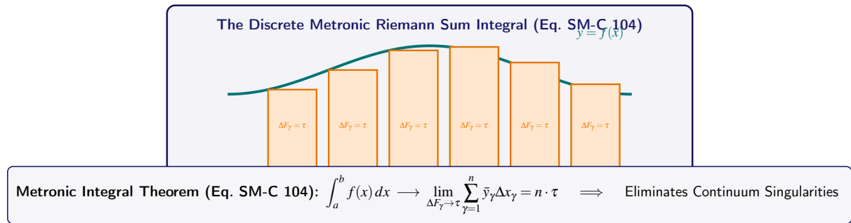
Figure 6.4. The Discrete Metronic Integral: Replacing continuous Riemann integration with finite cell summations scaled by the Weltmetron area \Delta F_\gamma = \tau .
