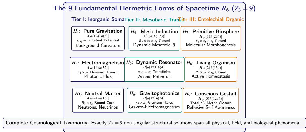
Figure 7.6. The 9 Fundamental Hermetic Forms of the Aeonic Universe ( Z_3 = 9 ): Spanning Inorganic Matter ( H_1 – H_3 ), Mesobaric Field Transits ( H_4 – H_6 ), and Entelechial Living Systems ( H_7 – H_9 ).
