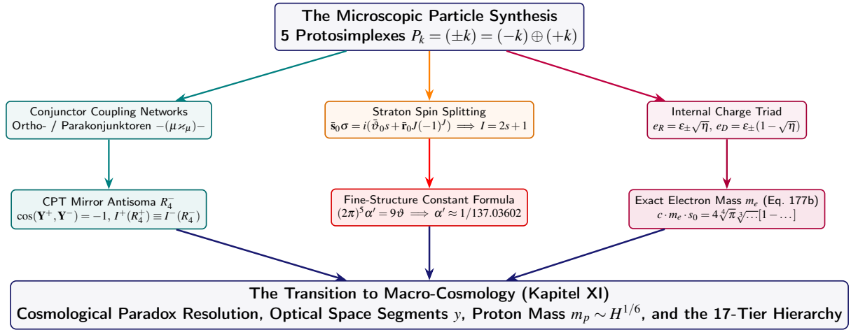
Figure 10.6. The Conceptual Deduction Tree of Chapter X: From Protosimplex flux isomerisms and Straton spin splitting to the exact electron mass m_e and fine-structure constant \alpha' .
