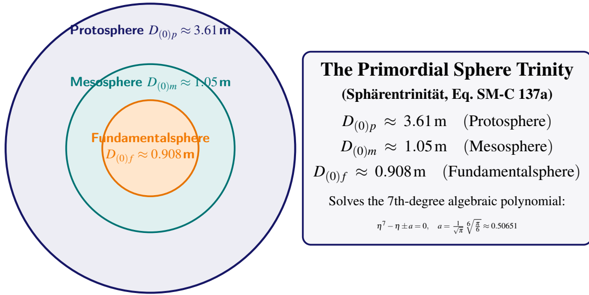
Figure 8.6. The Primordial Sphere Trinity of the Protouniverse: The monometronic initial state ( t = 0 ) from which cosmic expansion unfolds.
