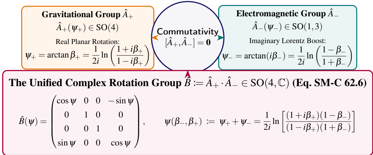
Figure 3.3. The Synthesis of the Unified Complex Lie Group \hat{B} \in SO(4, \mathbb{C}) : Commutative multiplication of the Euclidean rotation \hat{A}_+ and Lorentz boost \hat{A}_- .
