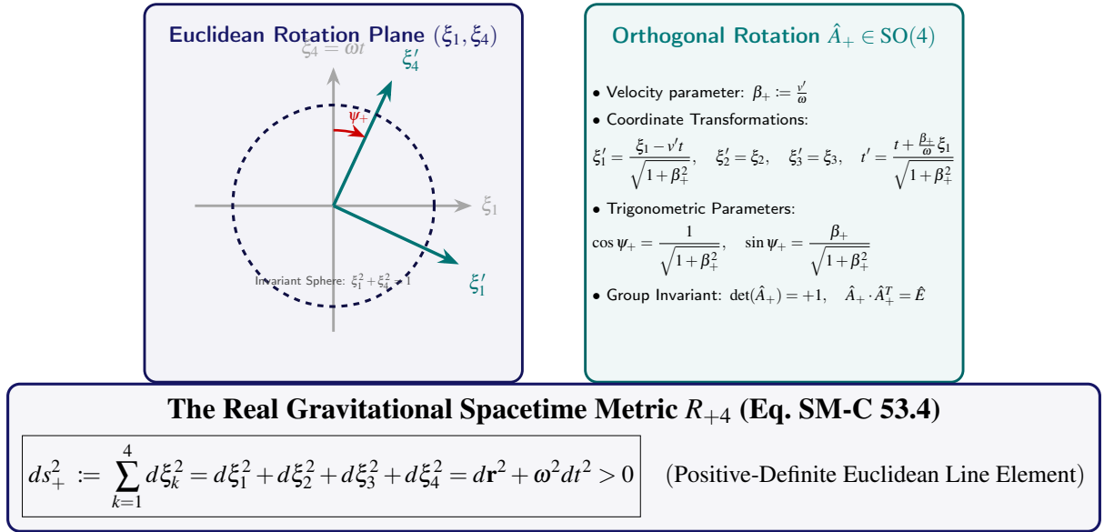
Figure 3.1. The Real Euclidean Gravitational Spacetime R_{+4} : Orthogonal spatial rotation of coordinate frames preserving the positive-definite metric ds_+^2 = d\mathbf{r}^2 + \omega^2 dt^2 .
