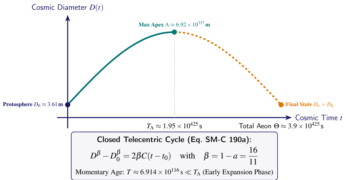
Figure 11.3. The Global Cosmogenetic Expansion Cycle: Symmetrical evolution from the Protosphere ( D_0 ) to the apex \Lambda and contraction to the final state D_e .
