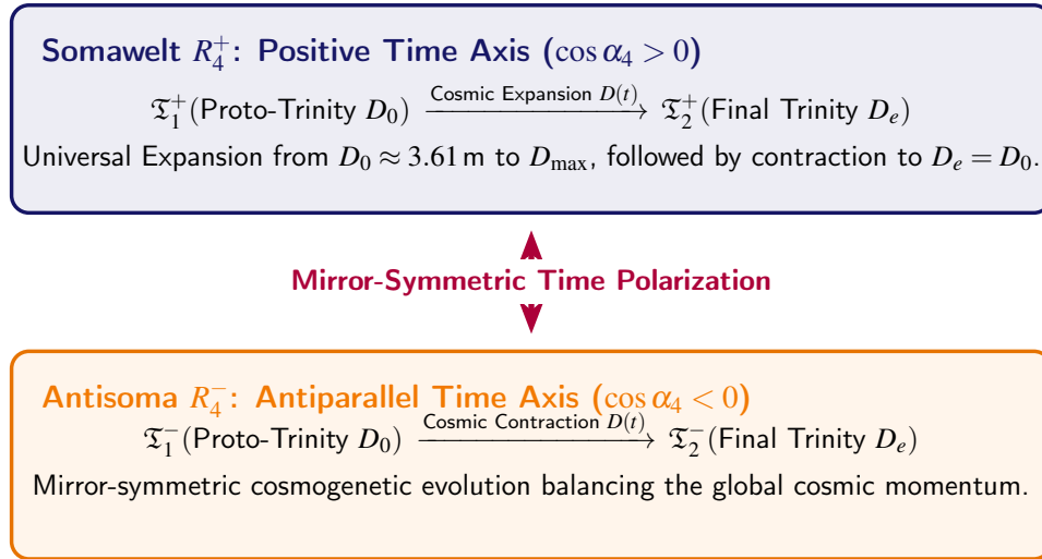
Figure 8.7. The Telecentric World Tectonics: Closed cosmogenetic cycle of the Somawelt ( R_4^+ ) and Antisoma ( R_4^- ).
