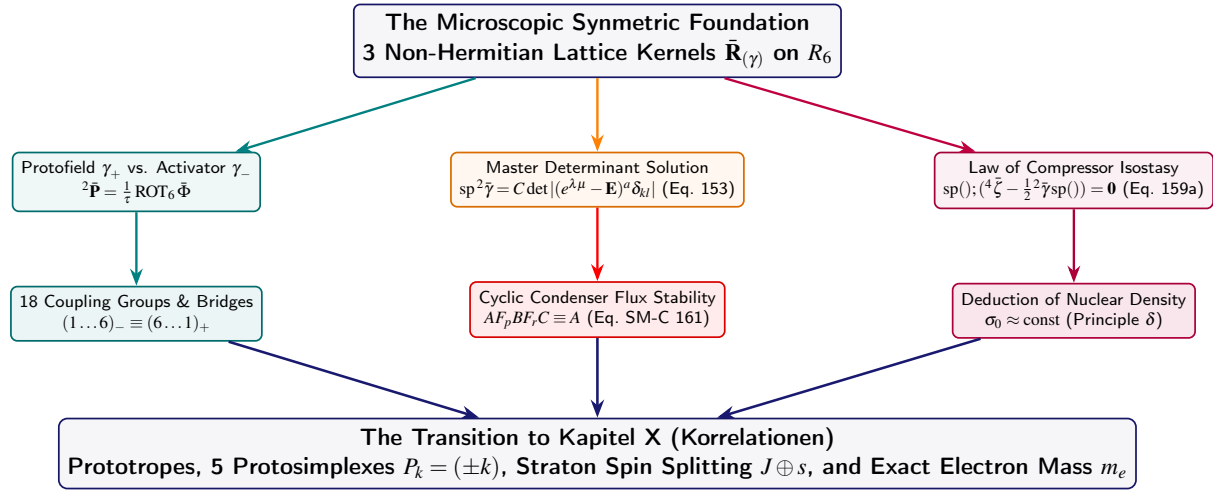
Figure 9.6. The Conceptual Deduction Tree of Chapter IX: From non-Hermitian lattice kernels and spinfield rotors to the Master Determinant Solution and Compressor Isostasy.
