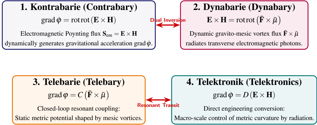
Figure 3.5. The Four Operational Modes of Field Correspondences: Unifying Contrabary, Dynabary, Telebary, and Telektronics into a closed electrogravitational transmutation loop.
