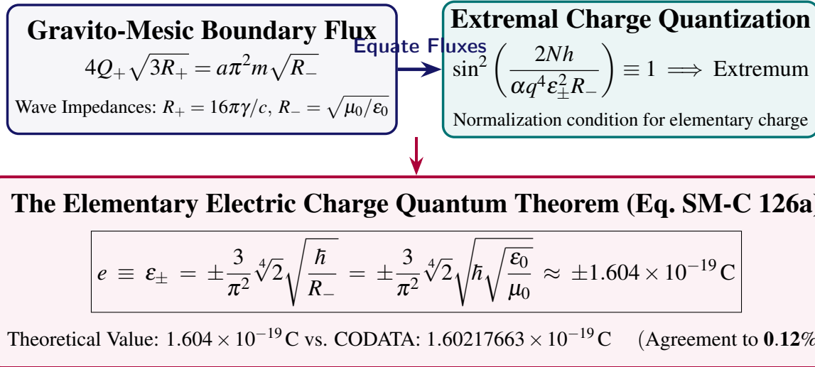
Figure 8.4. First-Principles Geometric Derivation of the Elementary Charge Quantum e : Linking Planck's constant \hbar and vacuum wave impedance R_- to deduce e \approx 1.604 \times 10^{-19} \text{ C} .
