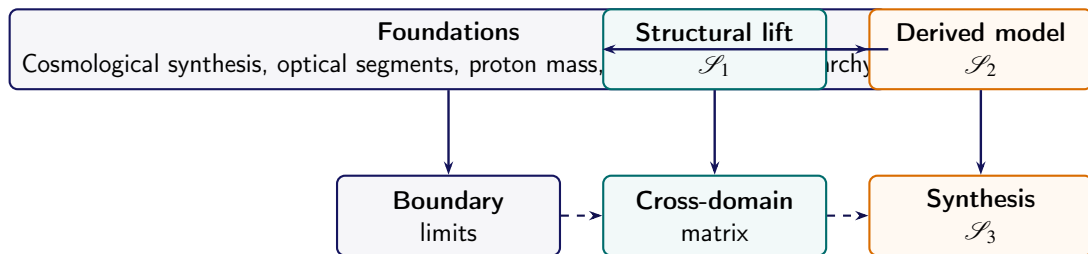
Figure B.1. Deductive progression of Chapter XI.
