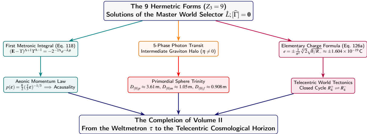
Figure 8.8. The Conceptual Deduction Tree of Chapter VIII: From the First Metronic Integral and elementary charge e to the Sphere Trinity and telecentric world tectonics.
