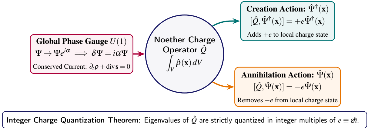
Figure 1.6. Noether Charge Operator Algebra: Global U(1) gauge invariance generating the quantized charge operator \hat{Q} and field ladder commutators.
