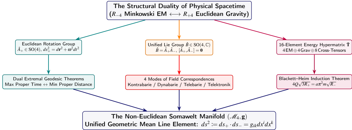
Figure 3.7. The Conceptual Deduction Tree of Chapter III: Somasynthesis of transformation groups, hypermatrices, field correspondences, and the Blackett–Heim theorem.
