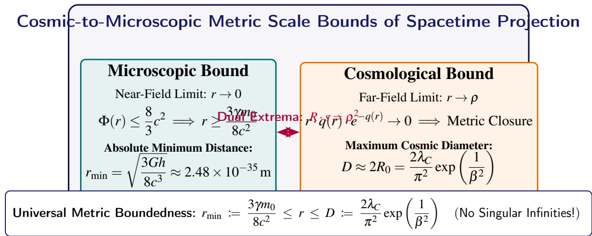
Figure 6.2. The Bounded Physical Continuum: The transcendental potential equation enforces an indivisible spatial floor r_{\min} at microscopic scales and a finite cosmological diameter D at large scales.
