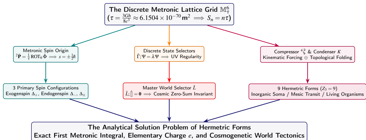
Figure 7.7. The Conceptual Deduction Tree of Chapter VII: From metronic spin hyperstructures and state selectors to the Master World Equation and the 9 Hermetric Forms.
