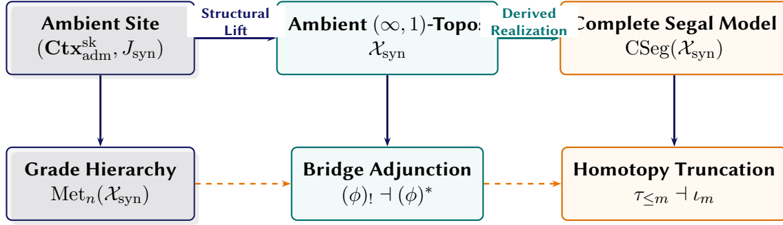
Figure 5.6. The Higher-Topos Tower, Change-of-Operad Adjunctions, and Tectonics in Chapter 5.
