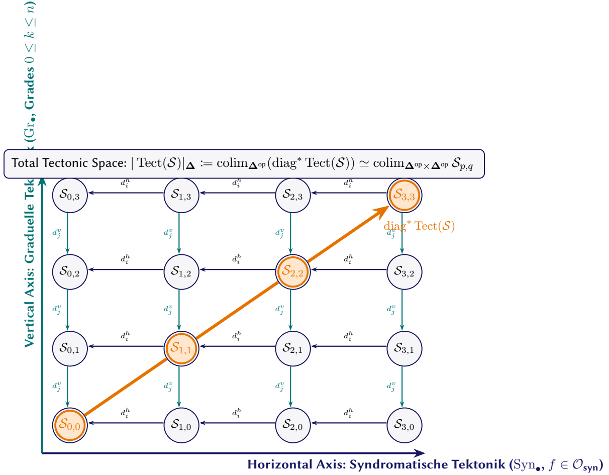
Figure 5.5. The Bisimplicial Tectonic Grid of an Associative Metroplex: Unifying Horizontal Syndrome Generation with Vertical Grade Nesting via Diagonal Geometric Realization.
