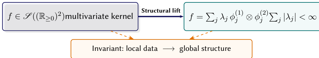
Figure 8.1. Nuclear Fréchet wave-packet spectral factorization..
