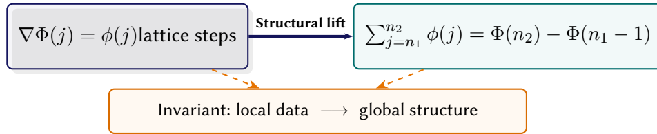
Figure 10.5. Discrete metronic telescoping fundamental-theorem staircase..
