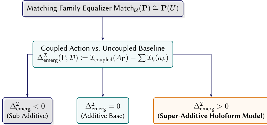
Figure 4.8. Classification of Sheaf Sections via the Coupling Non-Additivity Functional.
