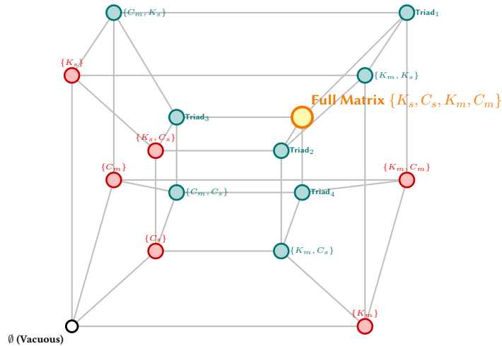
Figure 3.5. The 4D Tesseract Projection of the Corporate Rule Lattice: Visualizing the Topological Partition into 9 Determinate Mixed Operations vs. 6 Underdetermined Pure Stratum Pairs.
