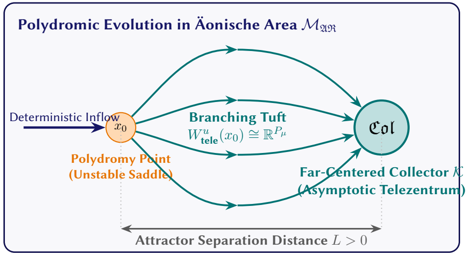
Figure 6.1. The Far-Centered Collector Bifurcation Cycle: An Unstable Polydromic Branching Tuft ( W^u(x_0) ) Reconverging Asymptotically into the Stable Basin of Collector Attractor \mathcal{K} .
