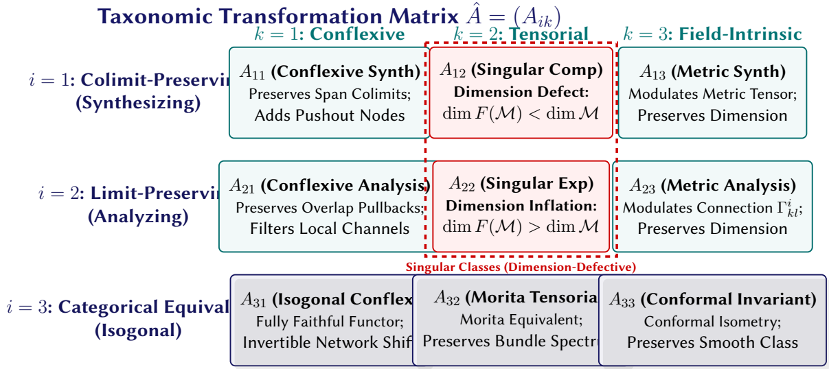
Figure 4.10. The Modernized Taxonomic Property Grid \hat{A} = (A_{ik}) : Classifying Field Transformations by Action Property ( i ) vs. Effect Target ( k ).
