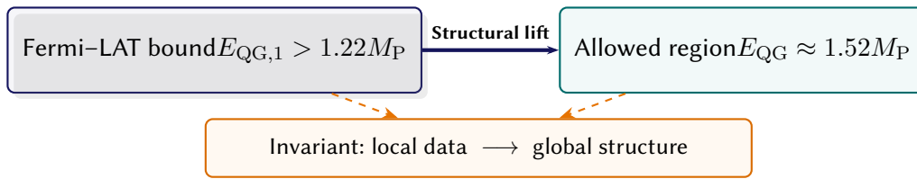
Figure 15.2. Astroparticle Lorentz-invariance-violation exclusion bounds..
