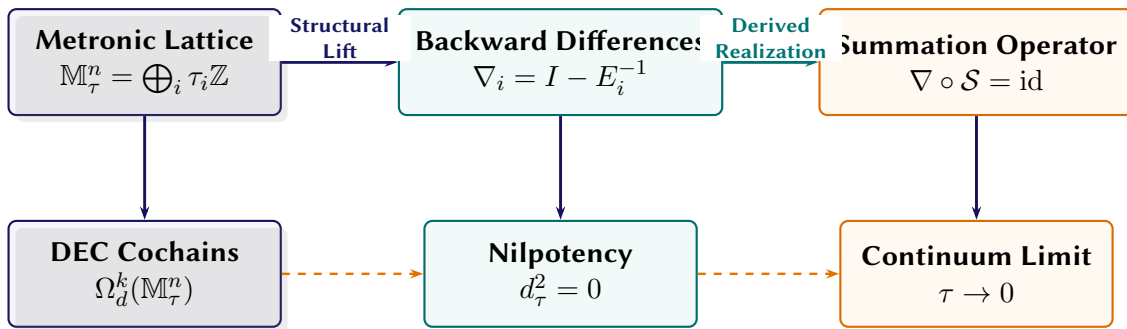
Figure 10.7. The Discrete Metronic Lattice, Difference Calculus, and DEC Topology in Chapter 10.
