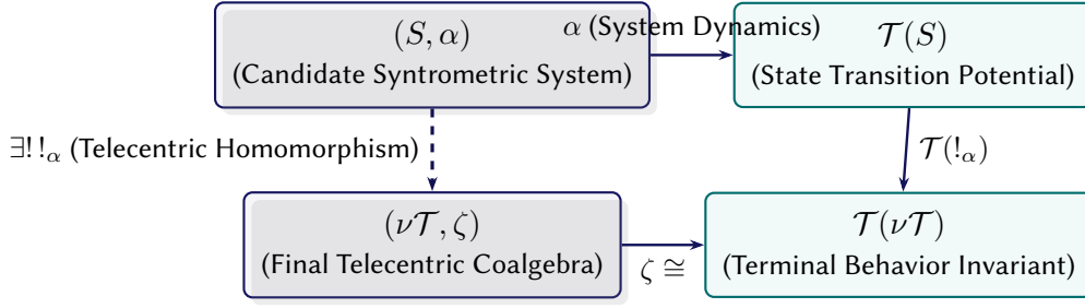
Figure 6.2. The Universal Telecentric Homomorphism to the Final Coalgebra (\nu\mathcal{T}, \zeta) .
