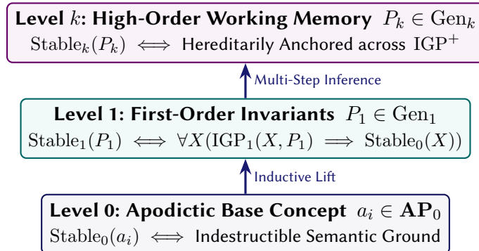
Figure 12.17. Working Memory Protection: The Hereditary Stability Modality Stable _k prevents representational drift across deductive strata.
