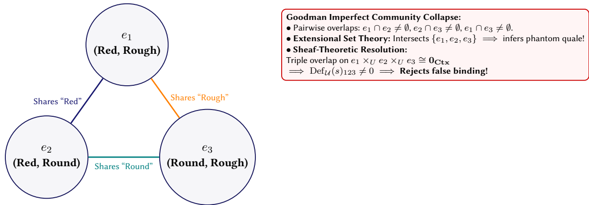
Figure 12.4. The Imperfect Community Problem and its Sheaf-Theoretic Resolution.
