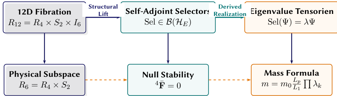
Figure 11.8. 12D Geometric Selectors, Null Stability, and Particle Mass Condensation in Chapter 11.
