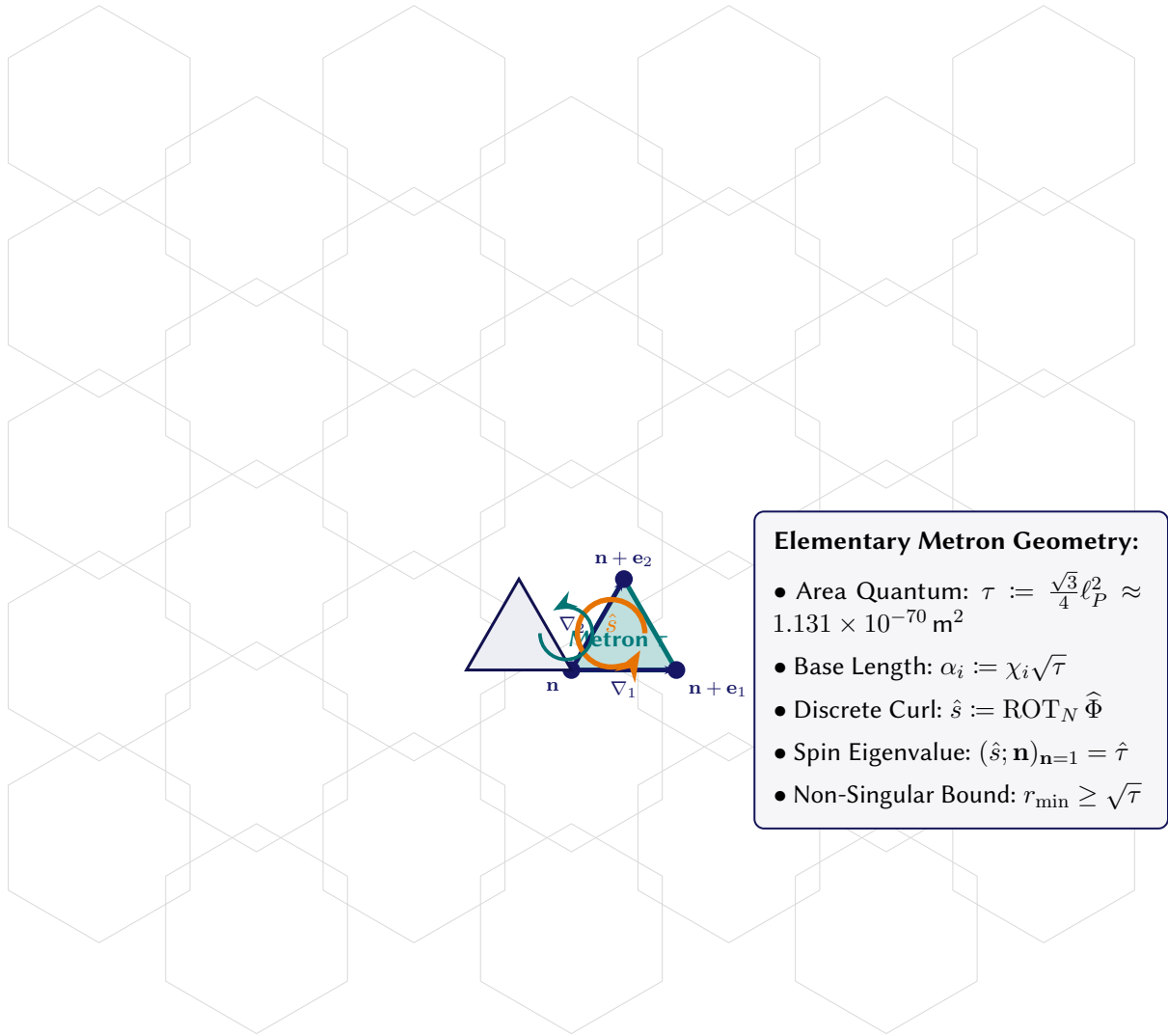
Figure 10.4. The Discrete Metronic Lattice Geometry: Fundamental Triangular Area Quantum \tau = \frac{\sqrt{3}}{4} \ell_P^2 with Backward Difference Stencils and Quantum Spin Rotor Vortices ( \hat{s} ).
