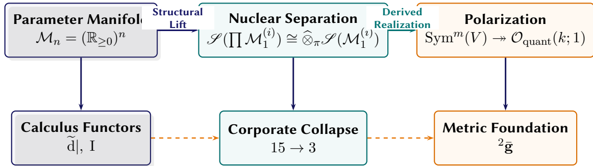
Figure 8.3. Nuclear Variable Separation, Homometral Reduction, and 3-Class Collapse in Chapter 8.
