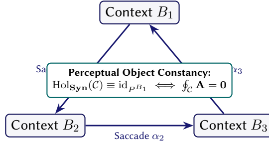
Figure 13.2. Metrophoric Holonomy Loop: Object constancy under active sensorimotor exploration.
