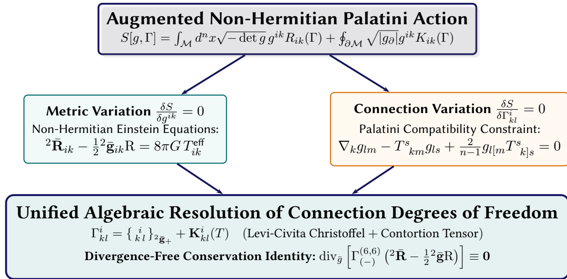
Figure 10.5. The Non-Hermitian Palatini Variational Framework: Independent Variation over Metric and Connection Determining the Contortion Tensor and Enforcing Covariant Conservation.
