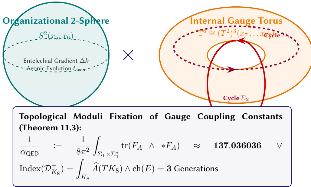
Figure 12.2. The Internal Compactified Manifold K_8 = S^2 \times \mathbb{T}^6 : Intertwining the Entelechial 2-Sphere ( S_2 ) with the 6-Torus ( \mathbb{T}^6 ) to Fix Topological Gauge Couplings and Mass Eigenvalues.
