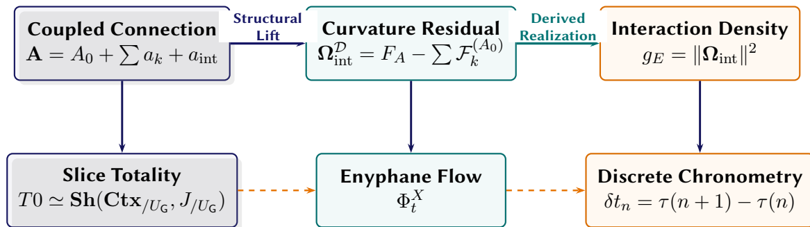
Figure 5.11. Non-Abelian Gauge Curvature, Diffeomorphism Flows, and Chronometry in Chapter 4.
