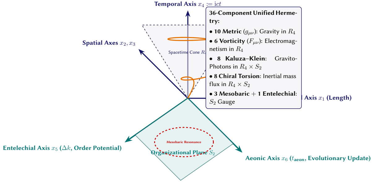
Figure 10.4. Geometric Projection of the 6-Dimensional Physical Subspace R_6 = R_4 \times S_2 : Metric Intertwining of Spacetime Kinematics with the Entelechial-Aeonic Organizational Plane.
