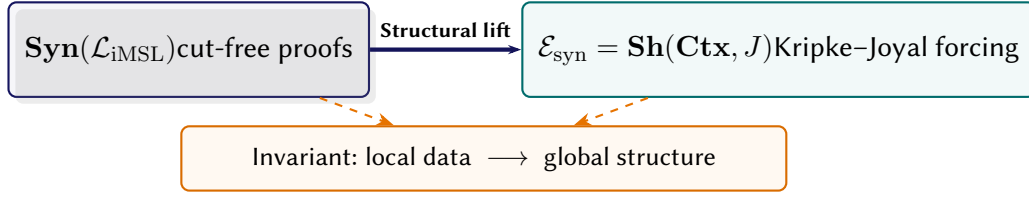
Figure A.2. Joyal topos representation functor from syntax to sheaf semantics..
