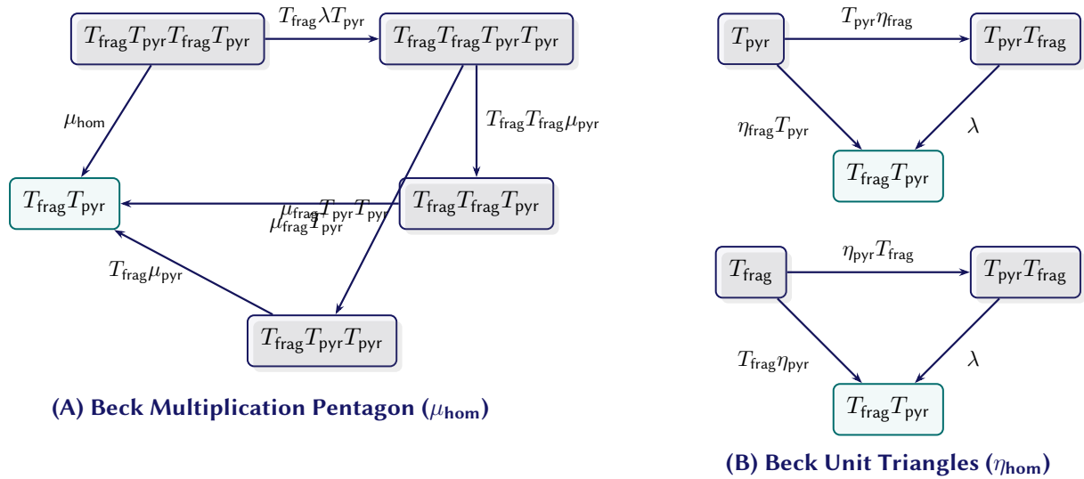
Figure 2.7. Beck Distributive Law \lambda: T_{\text{pyr}} \circ T_{\text{frag}} \Rightarrow T_{\text{frag}} \circ T_{\text{pyr}} Governing the Factorization of Homogeneous Syntrices (Spaltbarkeit).
