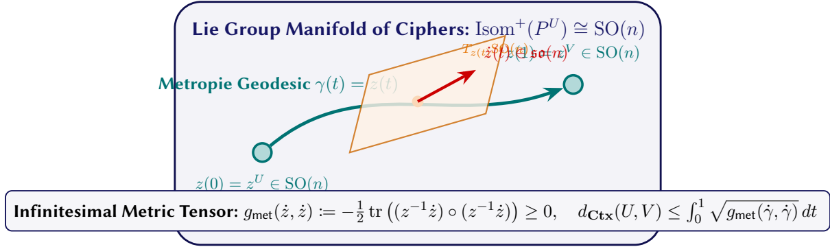
Figure 8.4. The Continuous Metropie Flow: Geodesic Trajectories across the Lie Group of Isometric Ciphers \text{Isom}(P^U) \cong \text{SO}(n) with Killing-Cartan Inner Product.
