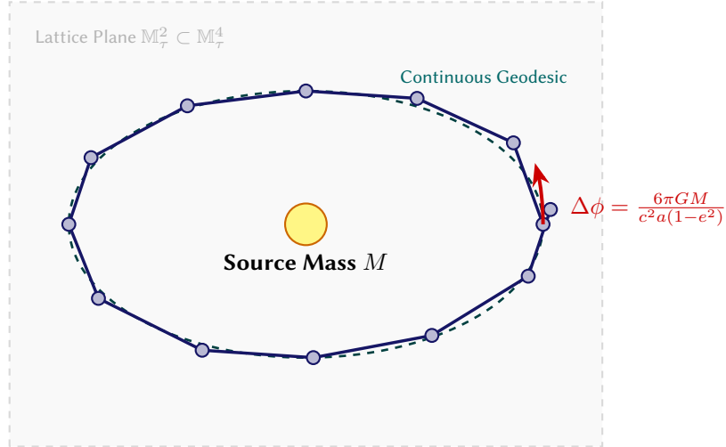
Figure B.2. Numerical Discrete Geodesic Integration on Lattice \mathbb{M}_\tau^2 : Precision Orbital Precession without Continuum Singularities.
