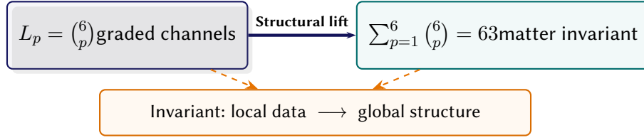
Figure 12.5. 63-channel matter-condensation hyper-lattice of R_6 .
