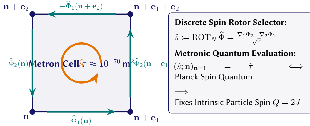
Figure 12.4. Discrete Spin Rotor Circulation on Elementary Metronic Cell \tau : Evaluating Discrete Rotor 2-Forms \hat{s} = \text{ROT}_N \hat{\Phi} to Fix Intrinsic Particle Spin Quantum Numbers.
