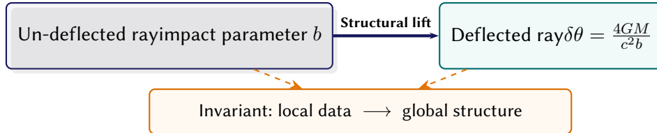
Figure B.3. Discrete gravitational light-ray bending on the metronic grid..
