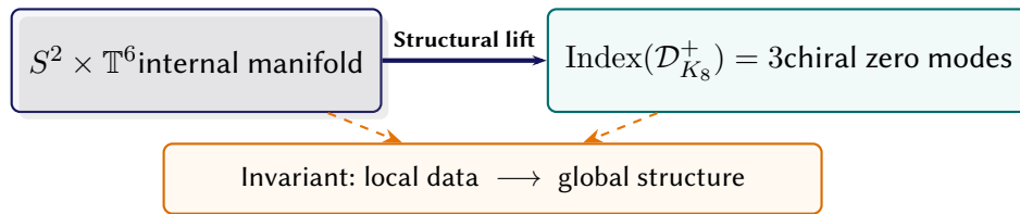
Figure 12.3. Topological three-generation Dirac index on K_8 = S^2 \times \mathbb{T}^6 .
