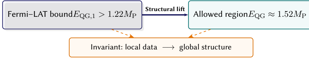
Figure 16.2. Astroparticle Lorentz-invariance-violation exclusion bounds..
