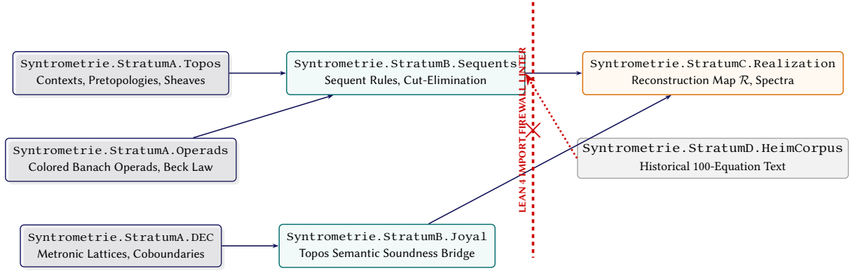
Figure C.1. Lean 4 Project Namespace Dependency DAG: The Transitive Dependency Firewall Statistically Prevents Physical Hypotheses (C) and Historical Manuscripts (D) from Entering the Formal Proof Core (A, B).
